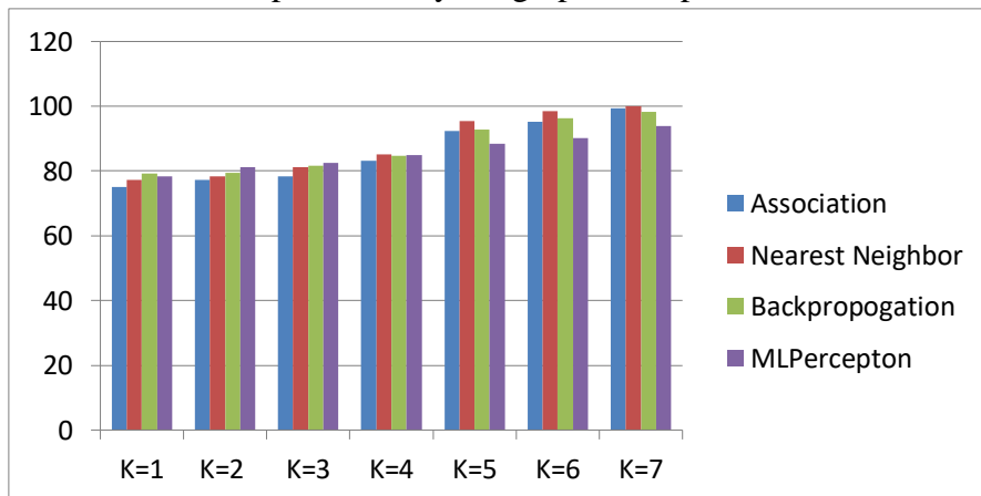
FIG.3: ACCURACY OF CLASSIFIER
